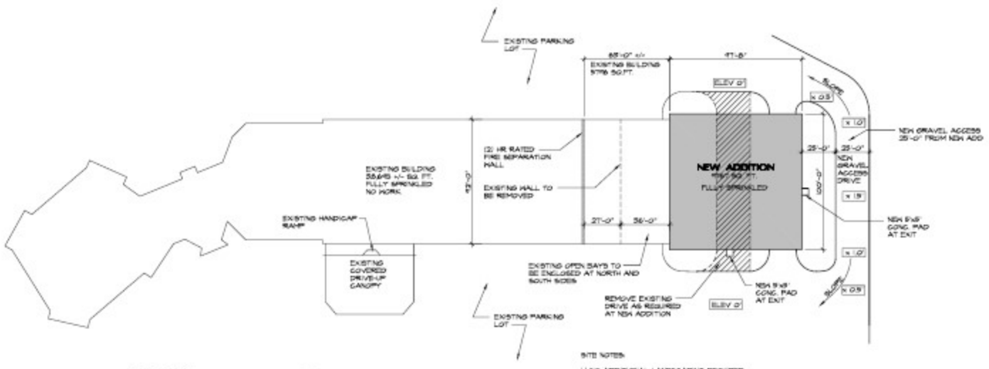
ARCHITECTURAL SITE PLAN SCALE = 1" = 40'-0"
